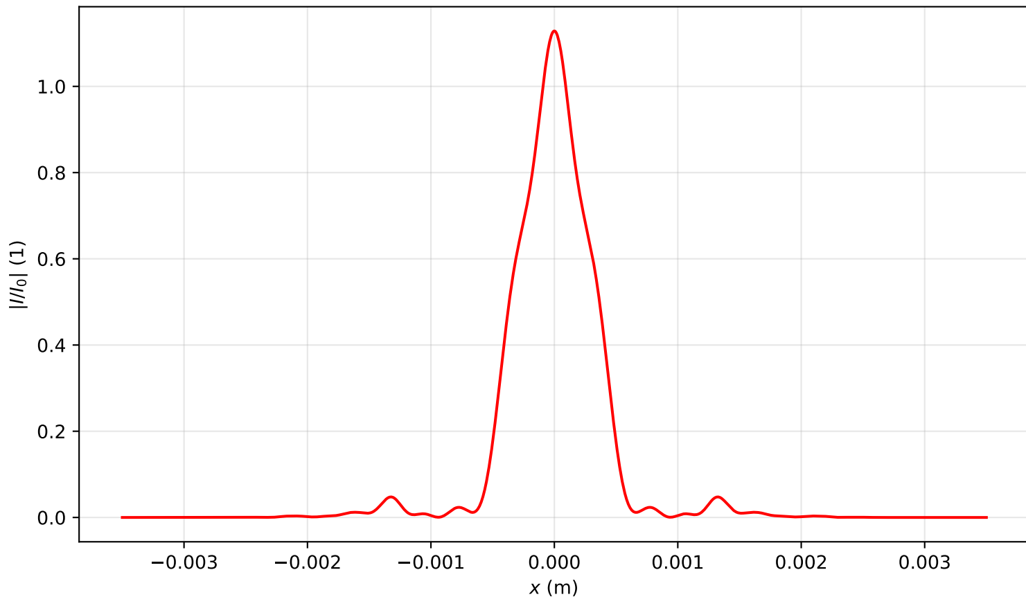
Intensity profile I(x, y = 0, z = 1.911)/I_0 , P_{in}=3.5P_{cr} , artificial time
